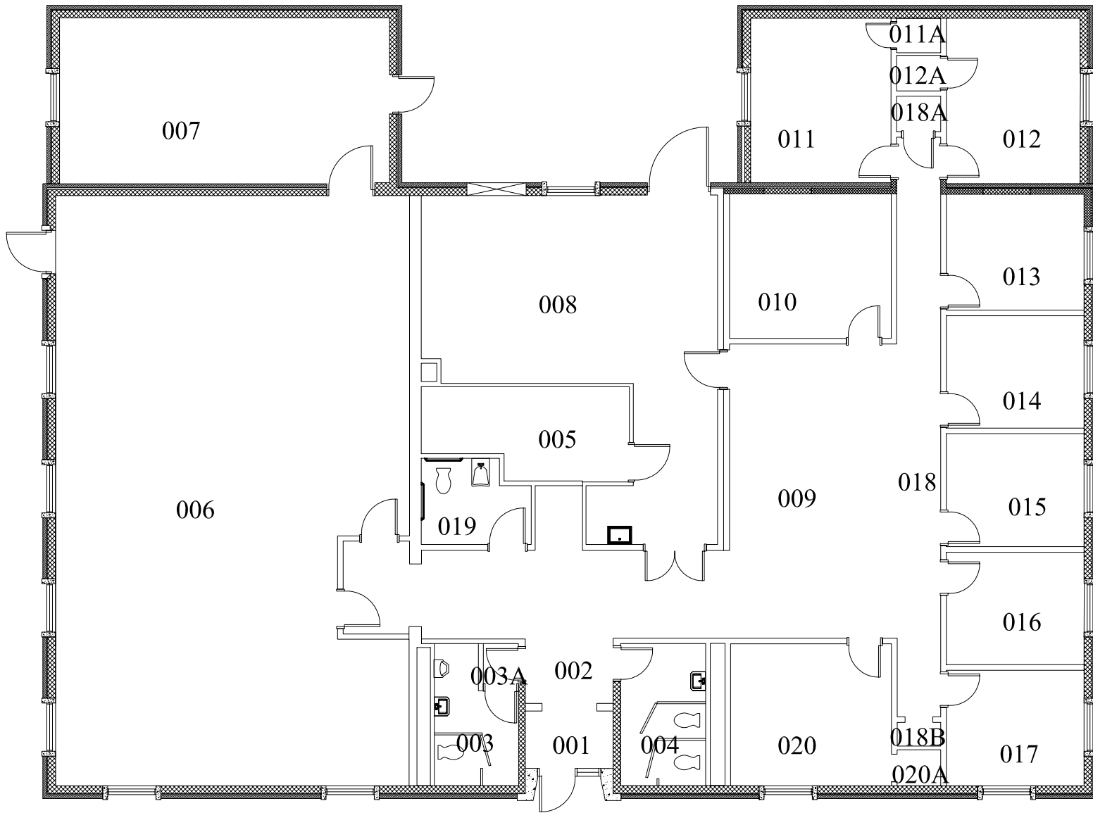
ALLEN COUNTY EXTENSION FIRST FLOOR NTS
