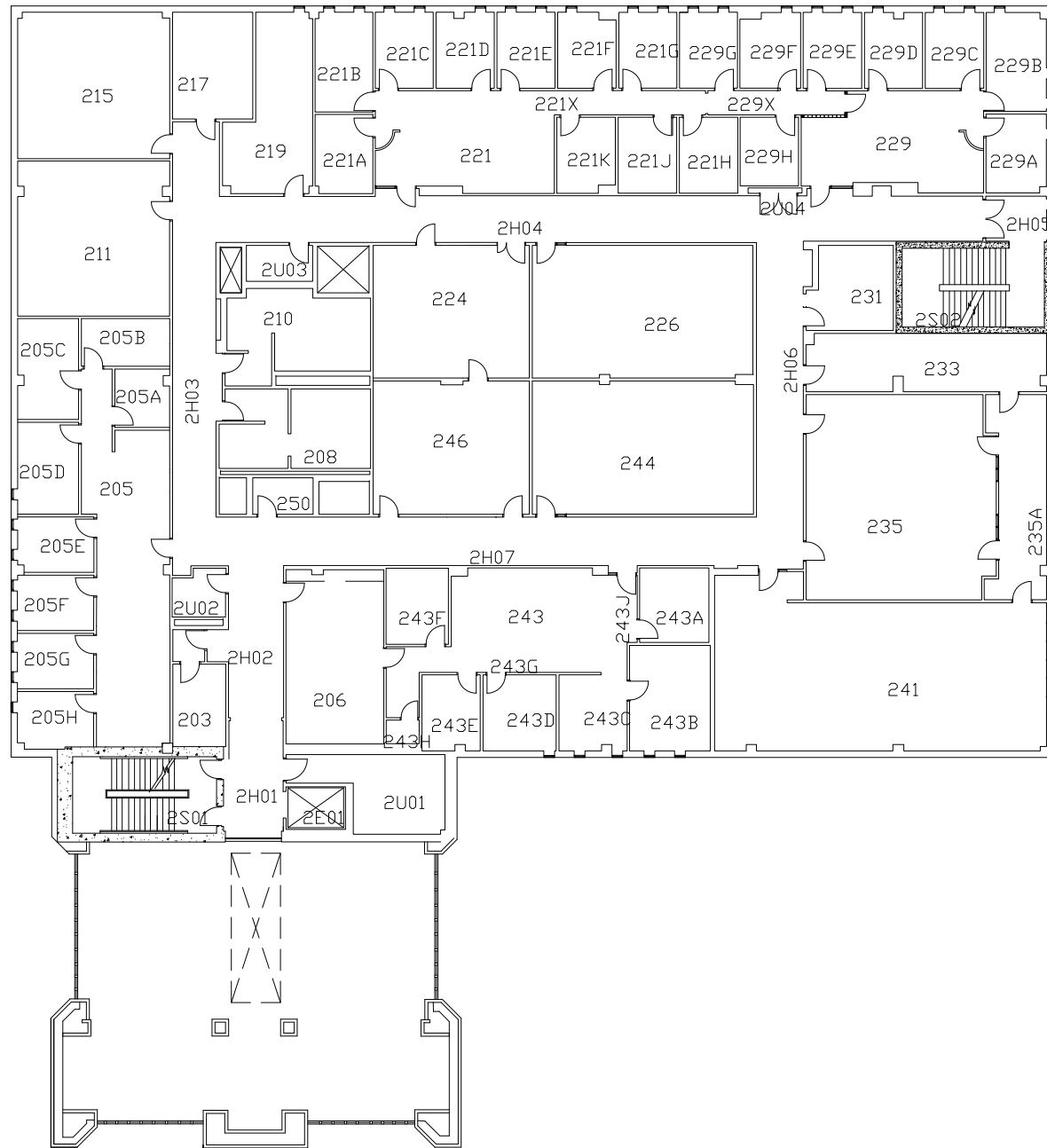
ENGINEERING & TECHNOLOGY SECOND FLOOR NTS
