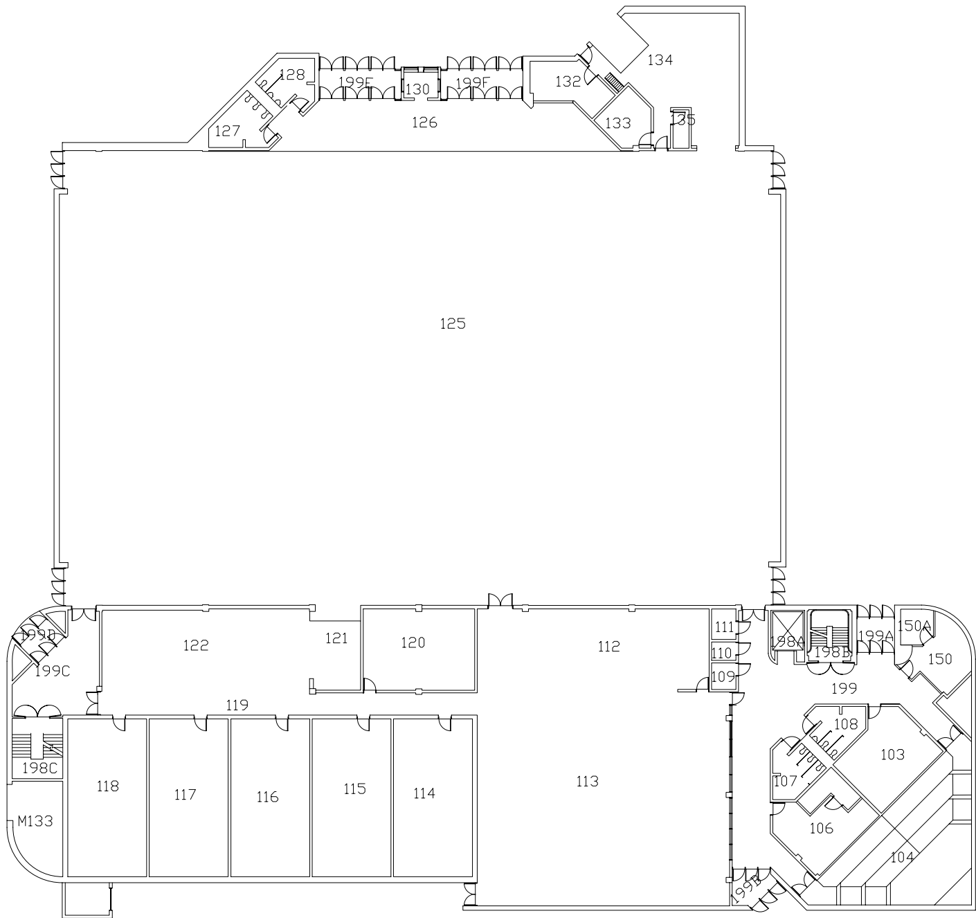
GATES SPORTS CENTER FIRST FLOOR NTS
